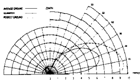
ELEVATION PATTERN (VOLTAGE) AT 2.5 MHz CURVES FOR VARIOUS TYPES OF GROUND
