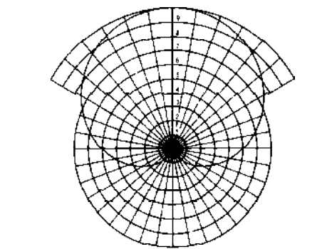
AZIMUTH PATTERN (VOLTAGE) FREQUENCY - 6 MHz
