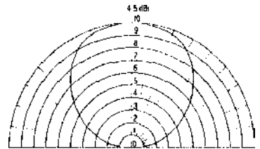
ELEVATION PATTERN F 15 MHz ST-230 SPIRAL ANTENNA CONDUCTIVITY 1E-03 DIELECTRIC CONSTANT 5 ODD MODE
