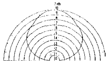
ELEVATION PATTERN F 27 MHz ST-230 SPIRAL ANTENNA CONDUCTIVITY 1E-03 DIELECTRIC CONSTANT 5 ODD MODE
