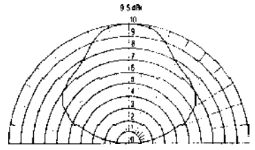
ELEVATION PATTERN F 2 MHz ST-230 SPIRAL ANTENNA CONDUCTIVITY 1E-03 DIELECTRIC CONSTANT 5 ODD MODE
