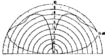
ELEVATION PATTERN F 2 MHz ST-230 SPIRAL ANTENNA CONDUCTIVITY 1E-03 DIELECTRIC CONSTANT 5 EVEN MODE
